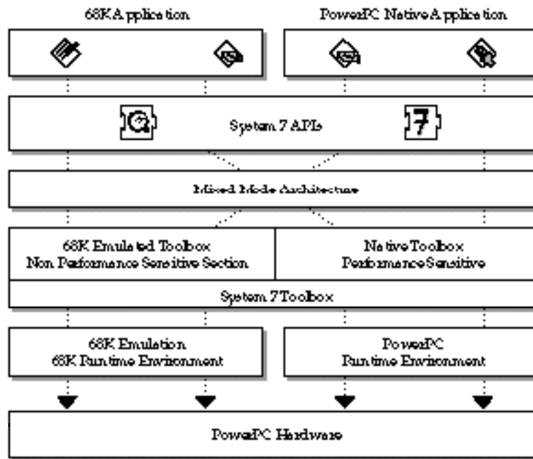
Macintosh on PowerPC Software Architecture
